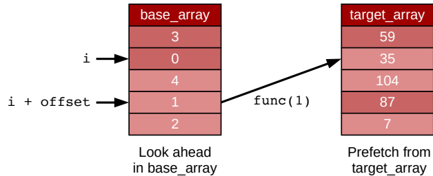
(b) Prefetching from target_array
